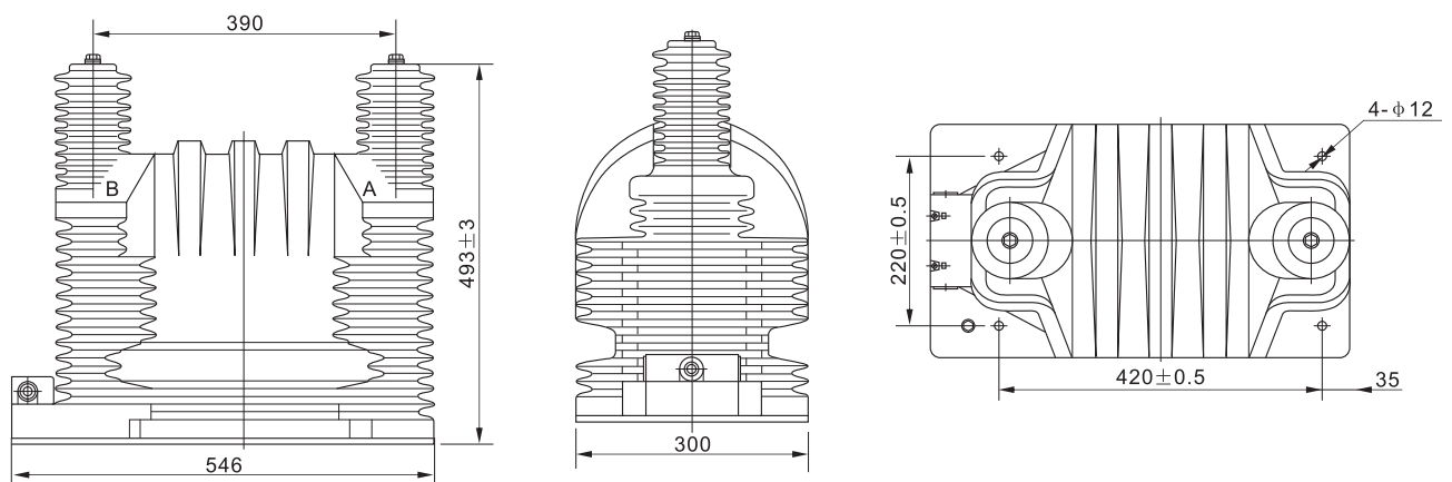
JDZ9-35Q Overall Dimension
