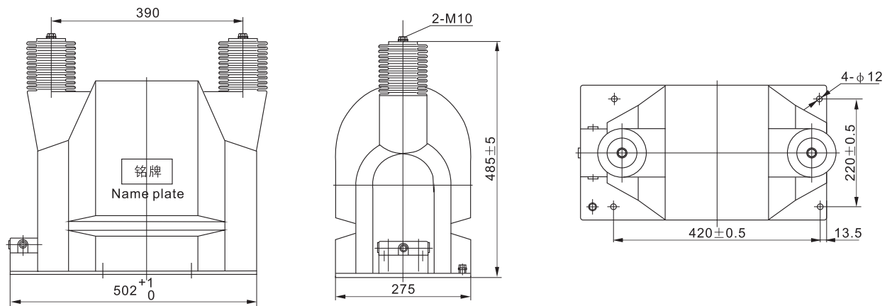
JDZ9-35 Overall Dimension
