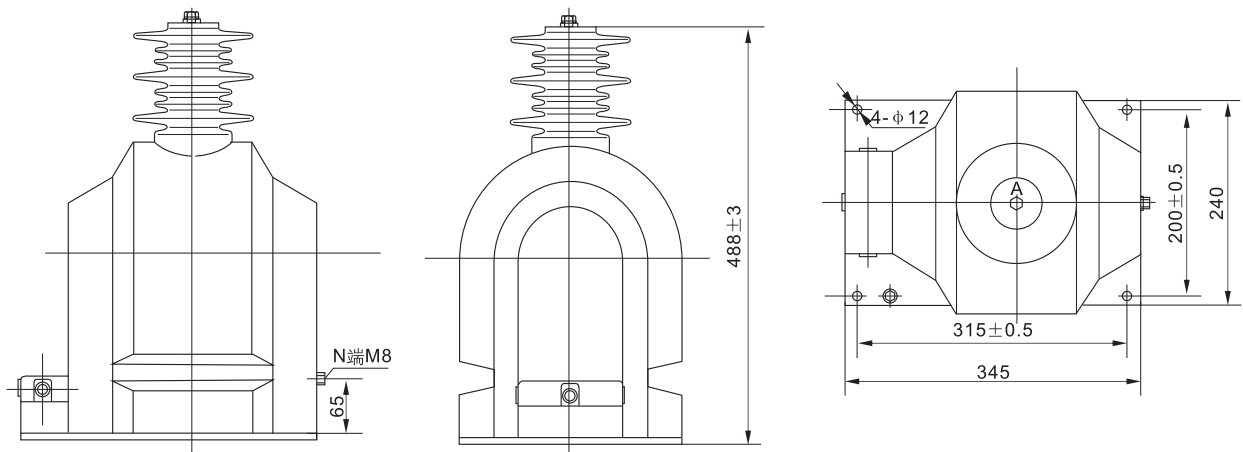
JDZX9-35Q Overall Dimension
